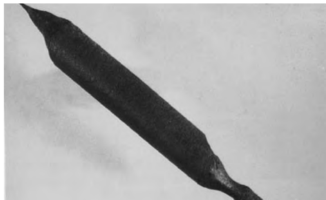
316L round bar 3/4 inch in diameter exposed to 1800°F (982°C). Air atmosphere. 316L is suggested to be used only to 1500°F (816°C), due to scaling. In contrast its melting point is 2540°F (1343°C).
