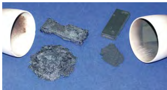
View of alloy 600 (left) and alloy 602CA (right) samples after 3000 hours at 2150°F (1177°C). Both samples began as 1/4" (6.3 mm) plate.
